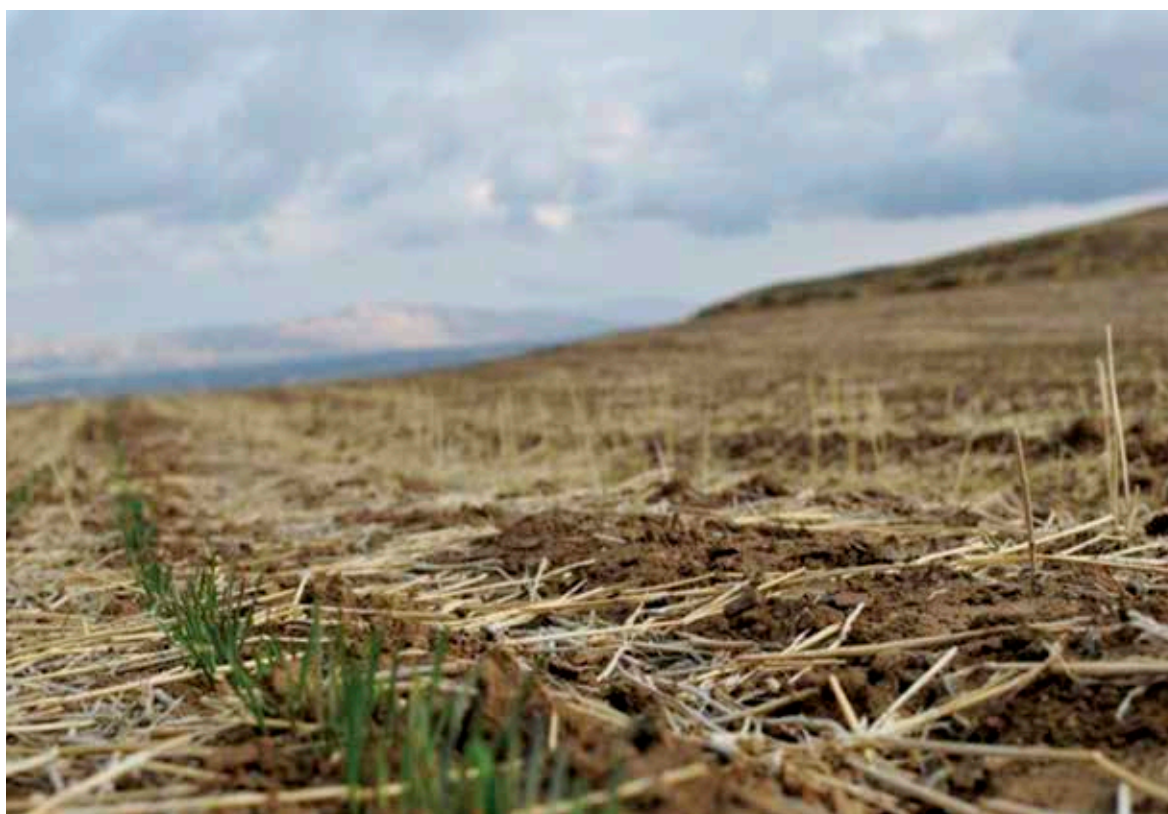
Figure 9. Soil protected by wheat residues, Tajikistan
