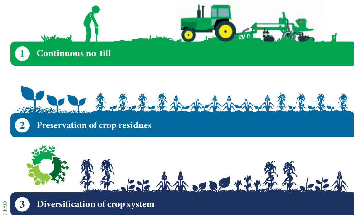
Figure 6. Three principles of conservation agriculture
