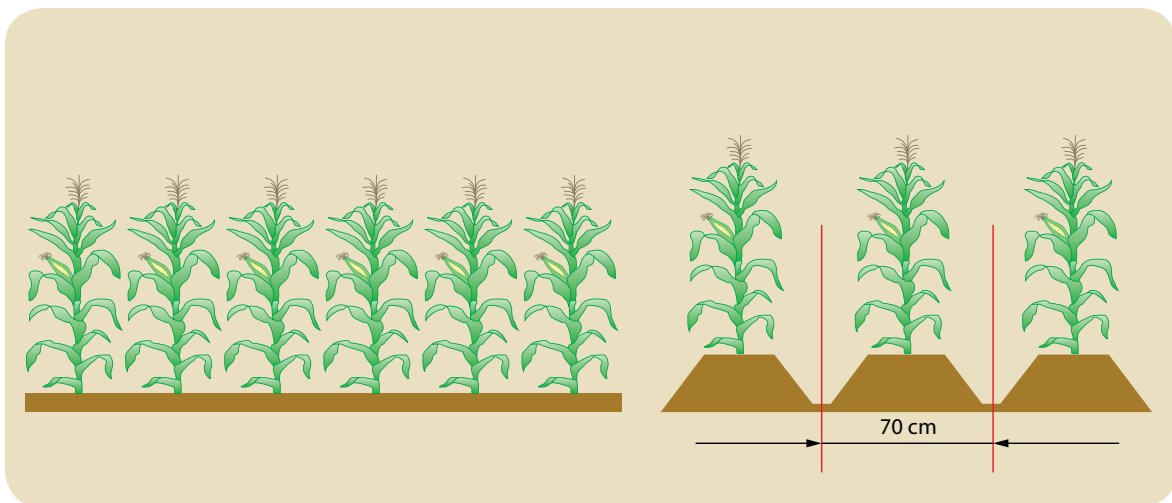
Figure 24. Configuration of conventional planting systems (left) vs raised beds (right)
