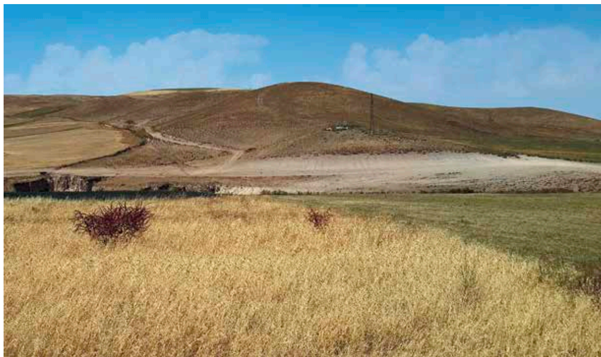
Figure 2. Example of slope erosion leading to gradual degradation of the soil
